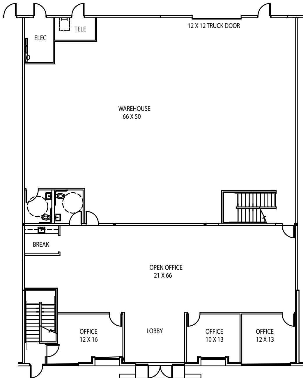
FIRST FLOOR
